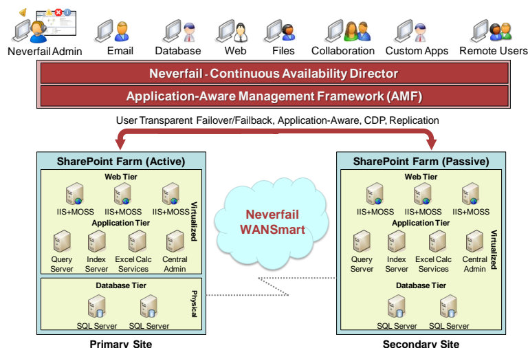
Figure 5: Neverfail WANSmart™
