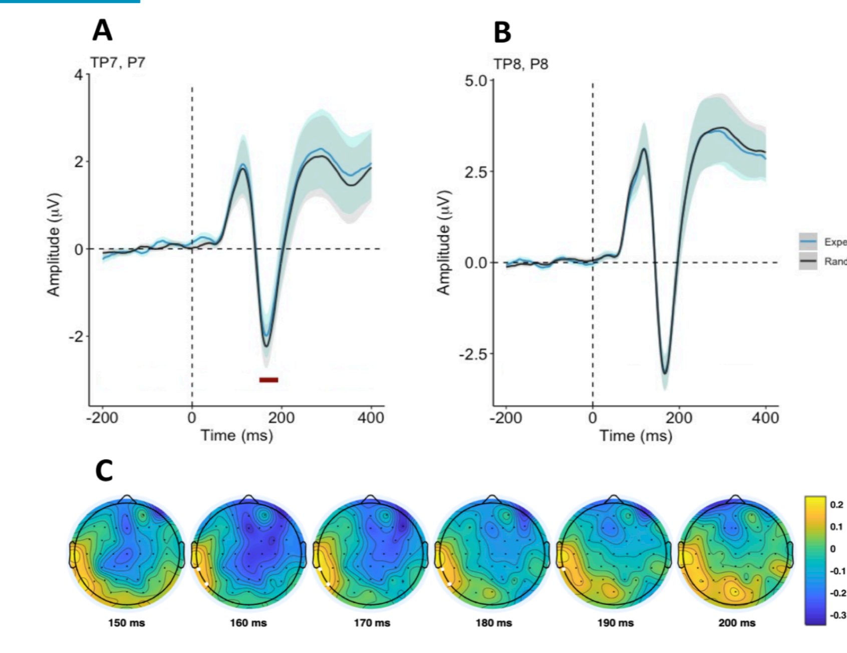
Figure 2. (A) A significant reduction in the N170 amplitude for expected (blue line) vs random (black line) faces was found across the averaged electrodes TP7 and P7 (left hemisphere; p = .003 , cluster corrected). The significant timeframe is marked by a dark red dash (152 – 192 ms). The shaded area illustrates within-participants confidence intervals for the expected (blue) and random (grey) faces. (B) The N170 illustrates no significant amplitude differences between the image categories across electrodes TP8 and P8 (right hemisphere; p > .05 , cluster corrected). (C) The topographies display the voltage difference ( \mu\text{V} ) between the expected and random face images in a timeframe from 150 to 200 ms after stimulus onset. A significant left-lateralised difference in amplitude extends from approx. 160 – 190 ms post-stimulus onset (electrodes highlighted in white).
