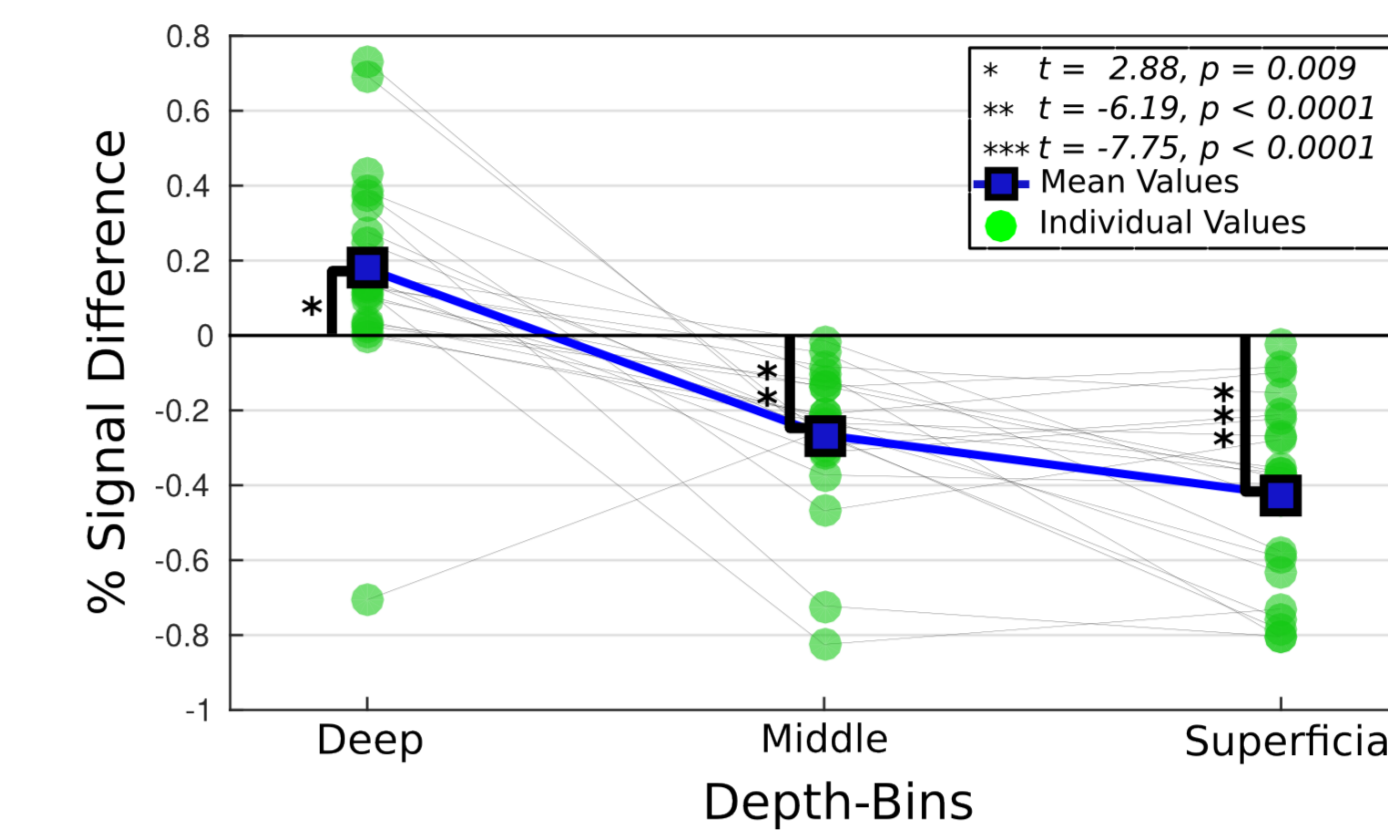
Real - Pseudo T-Scores (n=23) for group shown at each depth-bin 12
